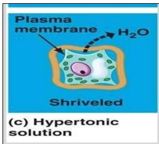
Plasmolysis
