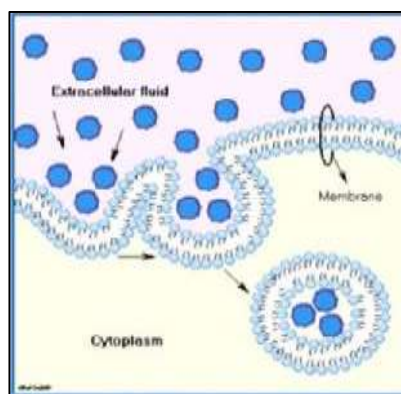
Absorption
