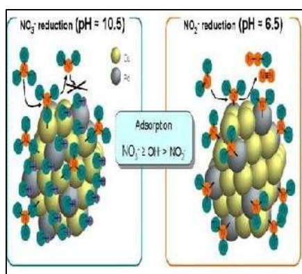
Adsorption
